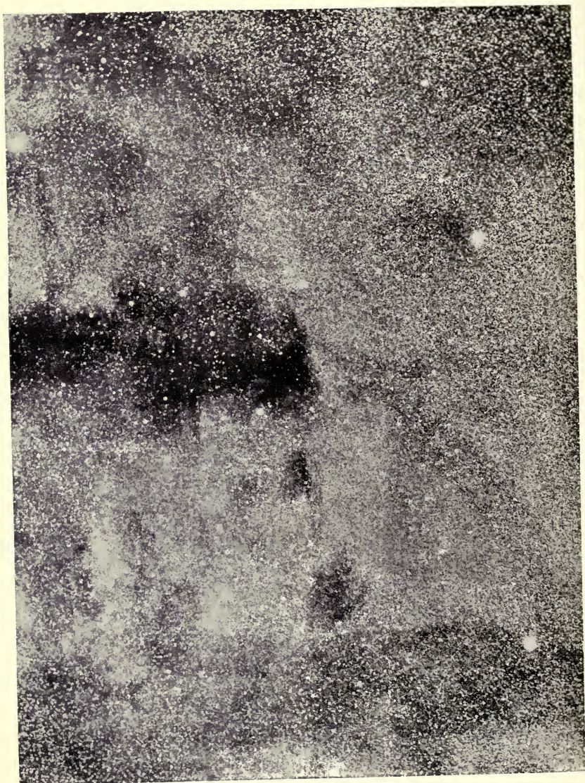
PHOTOGRAPH OF THE GREAT RIFT NEAR THETA OPHIUCHI.
