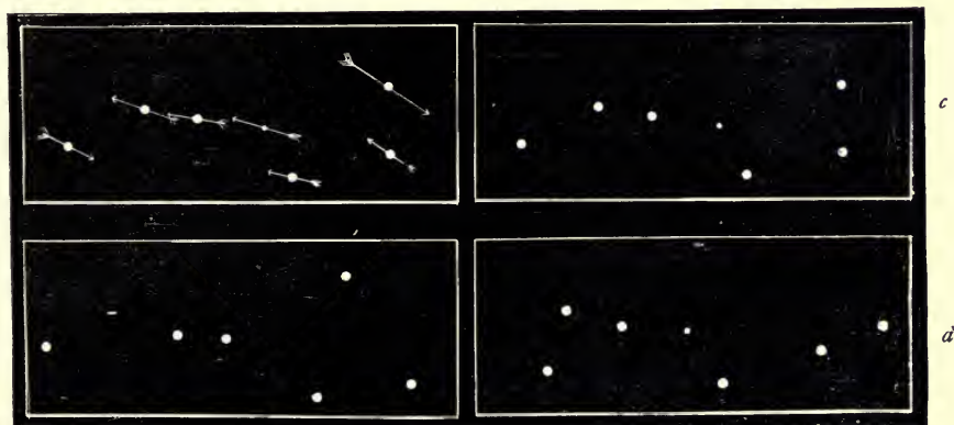
FIG. 2.—DRIFT OF THE STARS OF THE PLOUGH.
