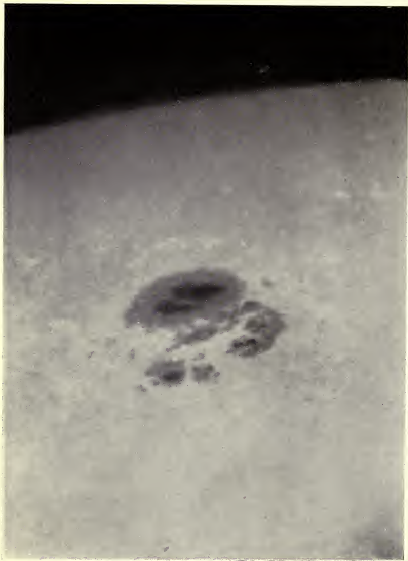
Photograph of a great group of Sun-spots, taken at the Royal Observatory, Greenwich, August 3, 1906. The group is the same as in PLATE XXV , but is now near the rim of the sun, and is seen foreshortened. The bright ridges are faculae.
