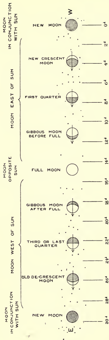
Moon's progress from west to east during a month, and corresponding change of phase.
