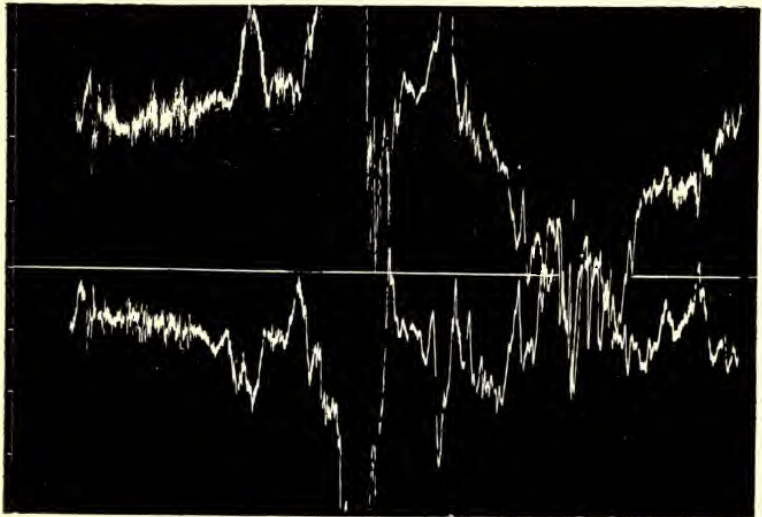
Horizontal Force. Declination. 1892, February 13 noon to February 14 noon.
