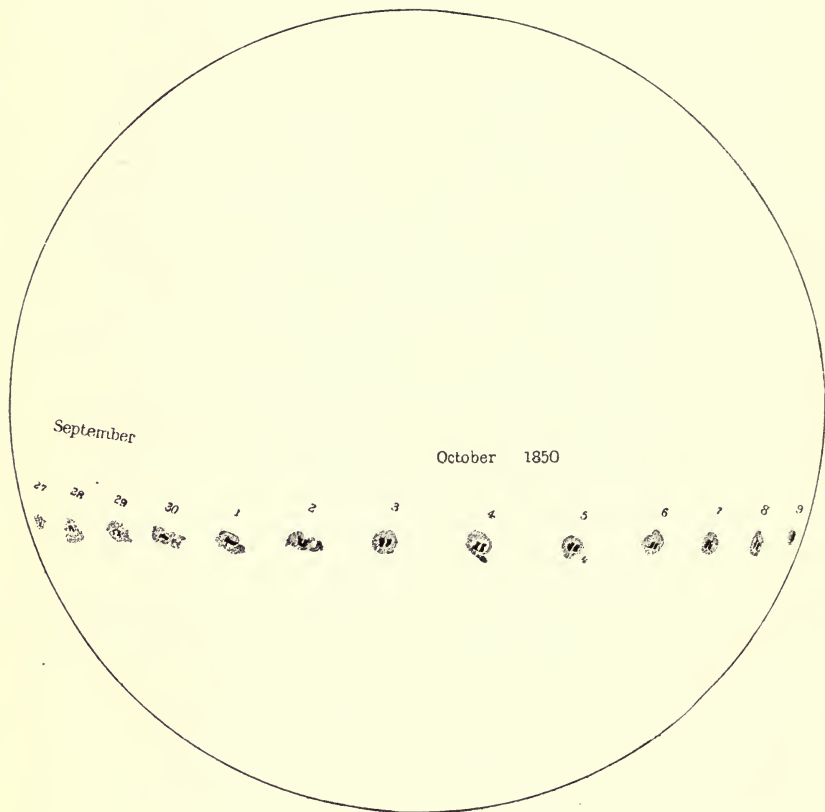
DIAGRAM SHOWING THE TRACK OF A SUN-SPOT ACROSS THE SUN'S DISC. (From a drawing made in September and October, 1850, by the late Father Sestini at the Georgetown College Observatory.)
