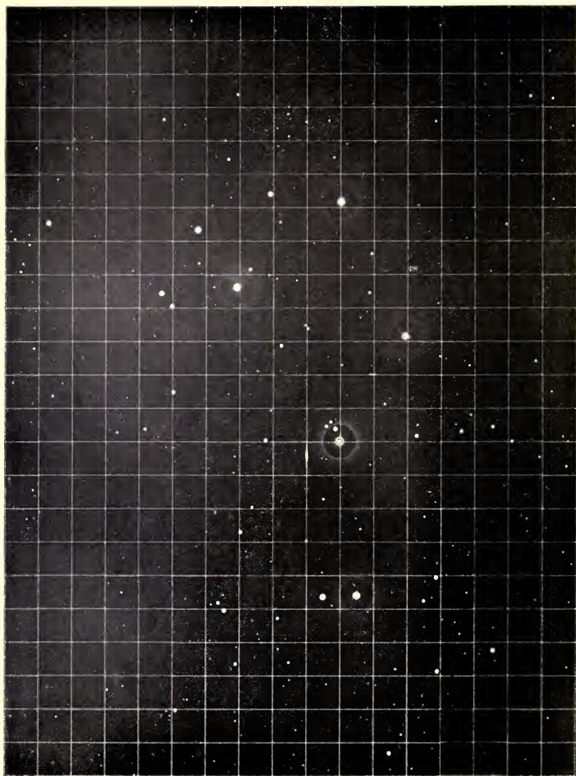
THE STARS OF THE PLEIADES. (Photographed with the 'Astrographic Telescope' of the Royal Observatory, Greenwich. Exposure, about 40 minutes.)
