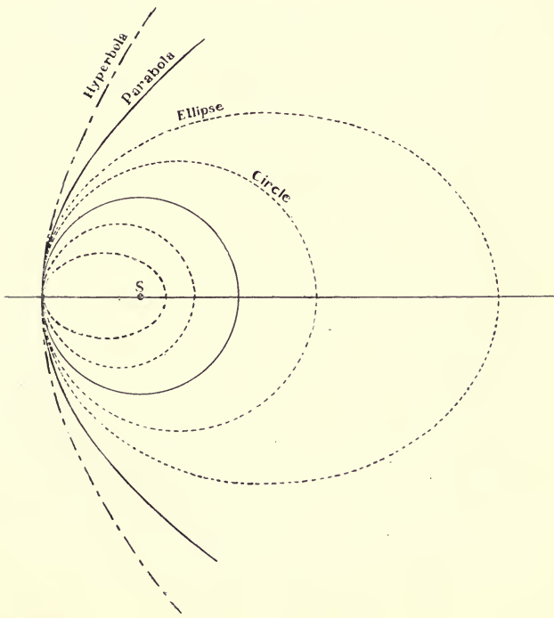
FIG. 1.—Forms of Cometary Orbits.
