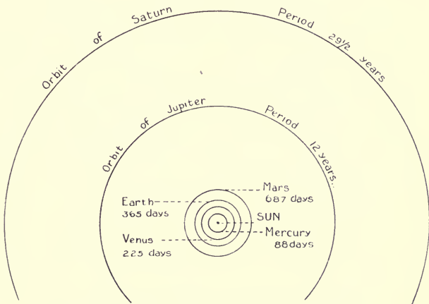
PLAN OF THE SOLAR SYSTEM
